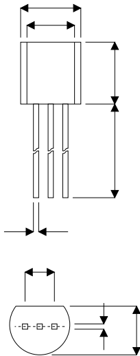
TO92 PACKAGE
